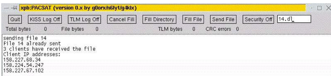
Figure 4. Modified xpb acting as server
